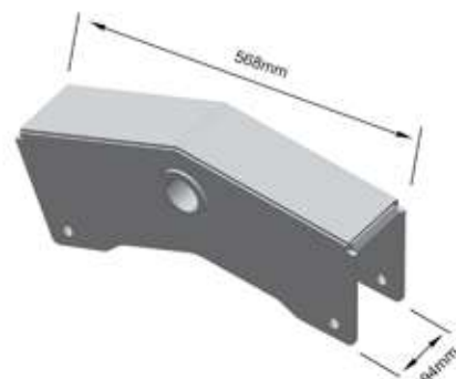
BALANÇA ASA DELTA SOLDADA P/PINO Ø 50,00mm P/CARREGA TUDO SP610 - ch. 8,00mm
