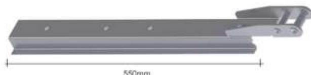
COLUNA SUPERIOR/INFERIOR DA GRADE MONTADA COM DOBRADIÇA SP350 SP770Z 450mm SP770D 900mm SP770 550mm SP770E 950mm SP770A 600mm SP770F 1000mm SP770B 700mm SP770G 1100mm SP770C 800mm
