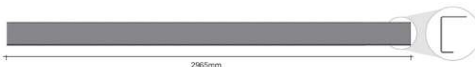
PERFIL LATERAL DA CARRETA SEM FURAÇÃO SP217 - 2965mm - ch. 4,25mm - 25,000kg SP217A - 2225mm - ch. 4,25mm - 18,760kg SP217B - 2430mm - ch. 4,25mm - 20,440kg SP217C - 2325mm - ch. 4,25mm - 19,600kg
