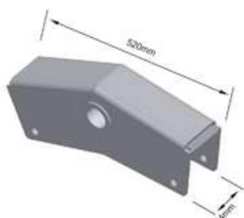
BALANÇA ASA DELTA ESTAMPADA P/PINO Ø 50,00mm - 2008 SP607 - ch. 8,00mm
