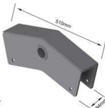
BALANÇA ASA DELTA SOLDADA P/PINO Ø 50,00mm P/CARRETA SP487 - ch. 8,00mm
