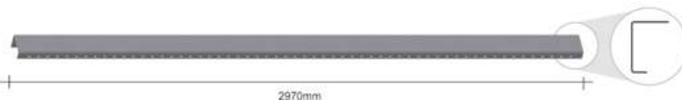
PERFIL LATERAL DA CARRETA COM FURAÇÃO SP794 - 2970mm - ch. 4,25mm - 25,000kg SP794A - 2230mm - ch. 4,25mm - 18,800kg SP794B - 2590mm - ch. 4,25mm - 21,840kg
