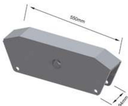
BALANÇA ASA DELTA SOLDADA P/PINO Ø 50,00mm TRUCK SP764 - ch. 8,00mm BALANÇA ASA DELTA SOLDADA P/PINO Ø 60,00mm TRUCK SP849 - ch. 8,00mm
